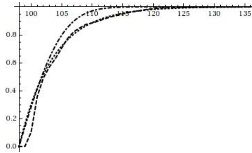
Figure 3: Experimental (dash), normal (dash-dot) and exponential (dot) CDFs, precise testing. Direction: Samara⇒Holland, W = 32 bytes
