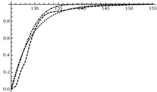
Figure 4: Experimental (dash), normal (dash-dot) and exponential (dot) CDFs, precise testing. Direction: Infolada⇒Athens, W = 32 bytes
