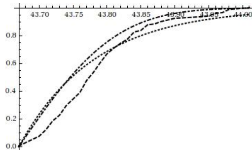
Figure 1: Experimental (dash), normal (dash-dot) and exponential (dot) CDFs, precise testing. Direction: tt01⇒tt143, W = 100 bytes
