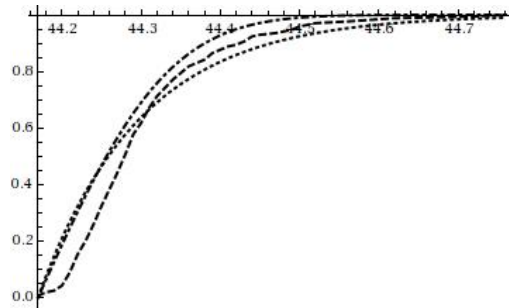
Figure 2: Experimental (dash), normal (dash-dot) and exponential (dot) CDFs, precise testing. Direction: tt01 \Rightarrow tt143, W = 1024 bytes
