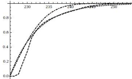
Figure 5: Experimental (dash), normal (dash-dot) and exponential (dot) CDFs, precise testing. Direction: SSAU \Rightarrow Australia, W = 1064 bytes
